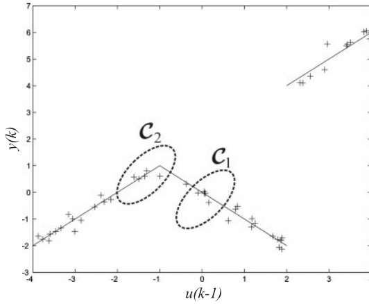
Fig. 1. The PWARX system (4) (-) and the dataset (crosses)
