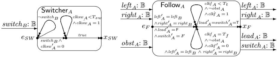
Fig. 6. Components \text{Switcher}_A and \text{Follow}_A
