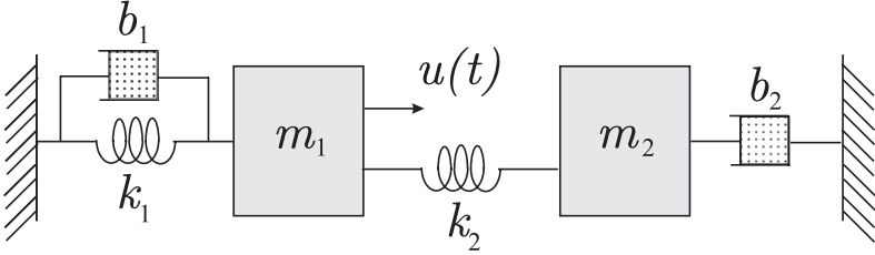
Fig. 4. Simple mechanical system.
