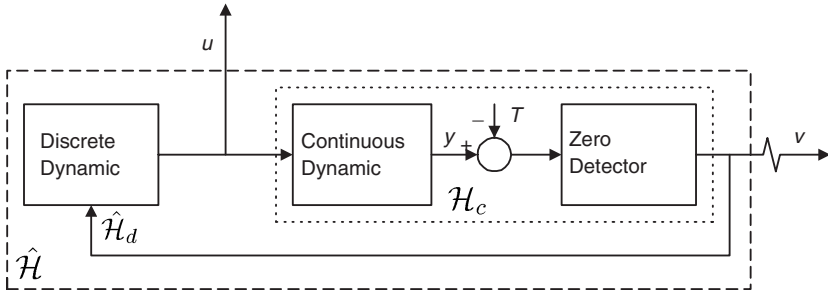
Fig. 1. Hybrid plant.
