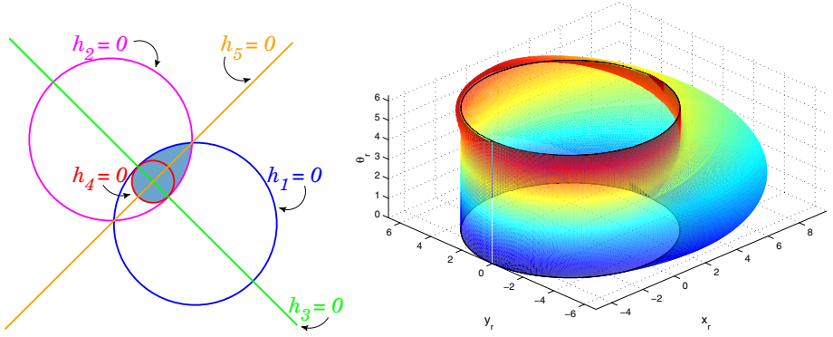
Fig. 1. Unsafe region for a given \theta_r Fig. 2. Maximal Controlled Invariant Set W^*
