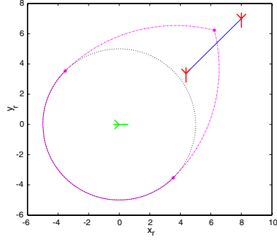
Fig. 4. Optimization without safety constraints over a shortened time horizon
