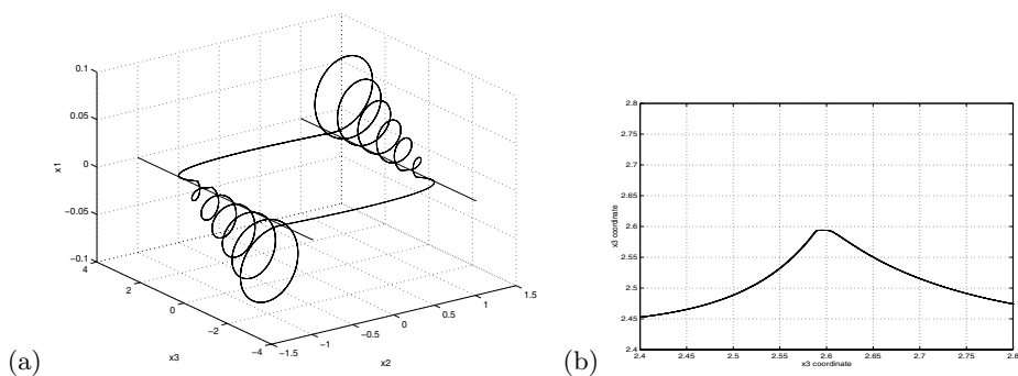
Fig. 8. Symmetric orbit with multiple amount of sliding sections (a) and corresponding 1-dimensional map (b)
