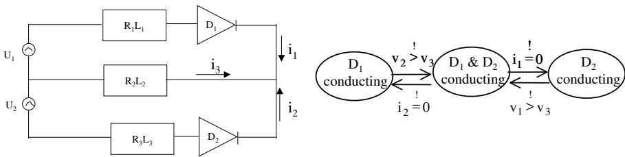
Fig. 5. Curcuit and state transition diagrams for Carver's example 3
