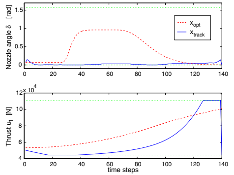
Fig. 8. Nozzle angle and thrust time histories
