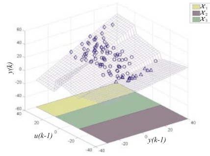
(b) Classified datapoints (triangles, diamonds, circles) and estimated model.
