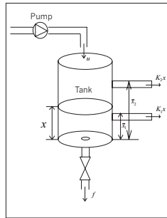
Fig. 1. Tank configuration
