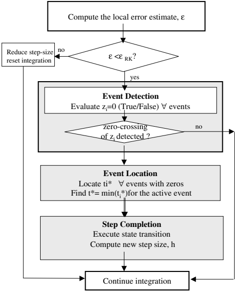
Fig. 1. Information flow diagram for integration with event-handling
