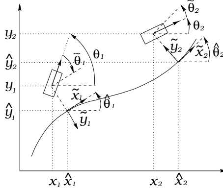
Fig. 1. Reference path and transformed coordinates.
