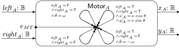
Fig. 2. Motor specification
