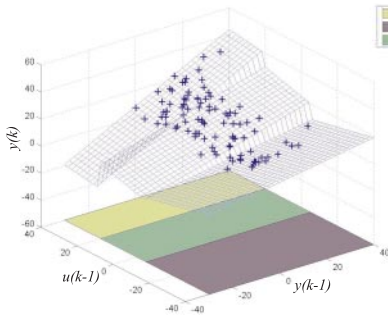
(a) The true model and the data-point (crosses)
