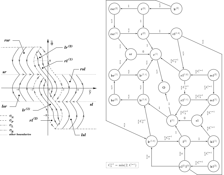
Fig. 5. On the left: shortest paths synthesis when d = 0 . On the right: quotient system FSM_{PTC} representing the behavior of the closed-loop hybrid system CLHA , when \sigma_r = \epsilon .
