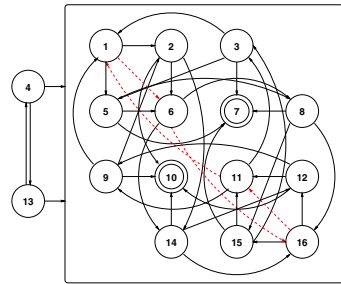
(b) Transition diagram for two cell automaton with zero boundary conditions.
