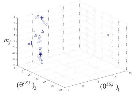
(b) Clustering of the vectors \xi_j with Algorithm 1. Clusters: triangle, diamonds, circles. The crosses are the centers of each cluster.
