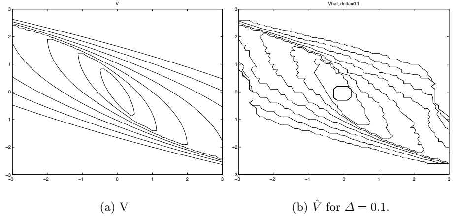
Fig. 2. Continuous and discrete value functions for double integrator
