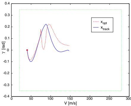
Fig. 9. Trajectories in (V, \gamma) Projection
