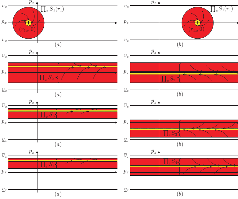
Fig. 4. Projection of S_1(r_1) , S_2(r_2) , S_3(r_3) , and S_4(r_4) onto: (a) p_x - \dot{p}_x plane; (b) p_z - \dot{p}_z plane
