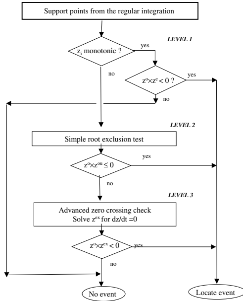
Fig. 2. Information flow diagram for hierarchical event detection
