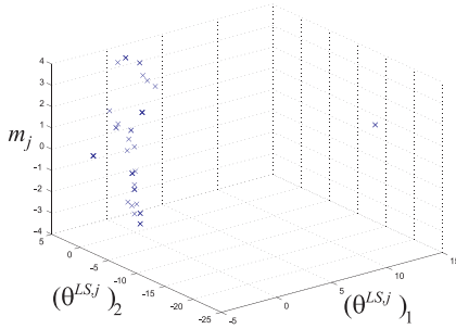
(a) The vectors \xi_j for the Example 1.
