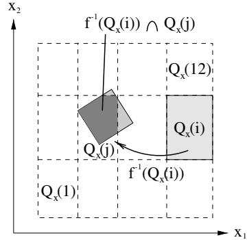
Fig. 3. Explanation of Ulam's method.
