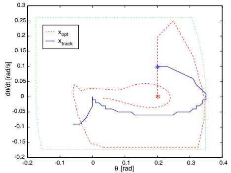
Fig. 10. Trajectories in (\theta, \dot{\theta}) Projection
