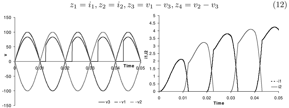
Fig. 6. (i) current profiles and (ii) voltage variations in the circuit problem
