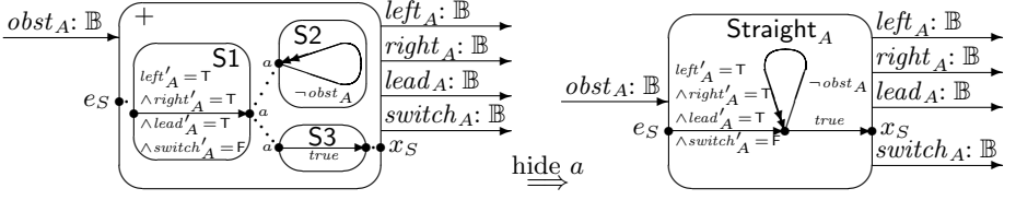
Fig. 3. Serial composition and location hiding
